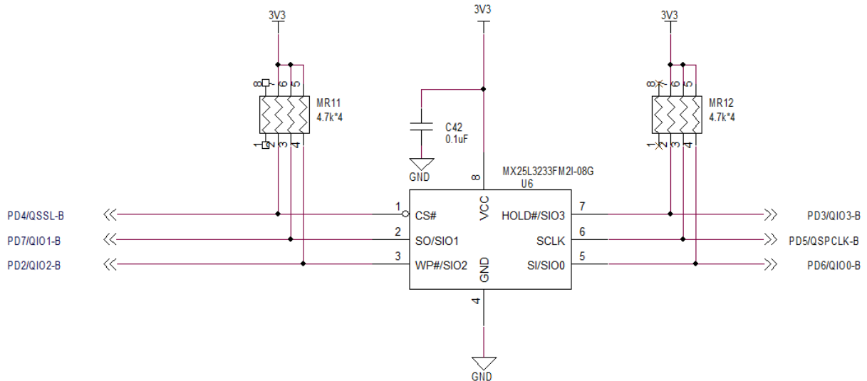
Figure 5-12. Serial Flash Connection Diagram
